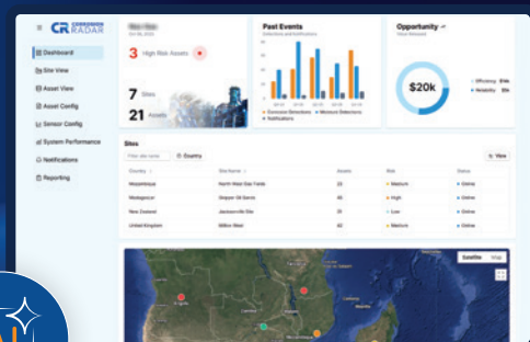
CR:CLARITY Dashboard
